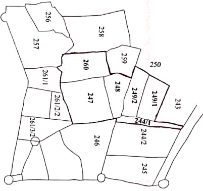
KHASRA MAP Scale - 1:4000
