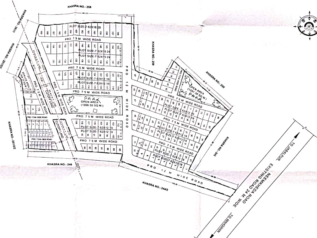
LAYOUT PLAN Scale - 1:1000
